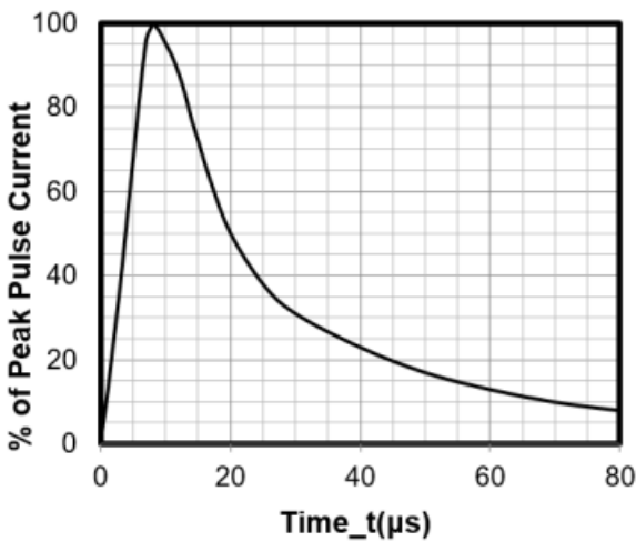
8 X 80μs Pulse Waveform
